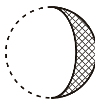
crescent moon
