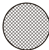
full moon
