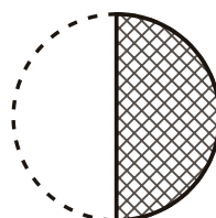
half moon
